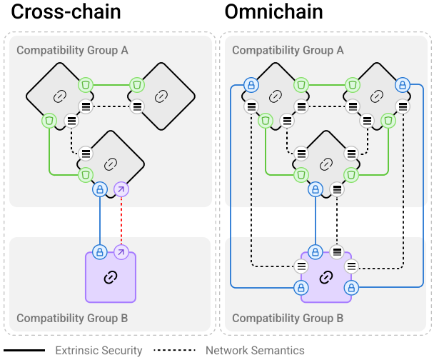
Figure 1: The omnichain fully-connected mesh network has universal network semantics for all connected chains and security specialized to each link.
