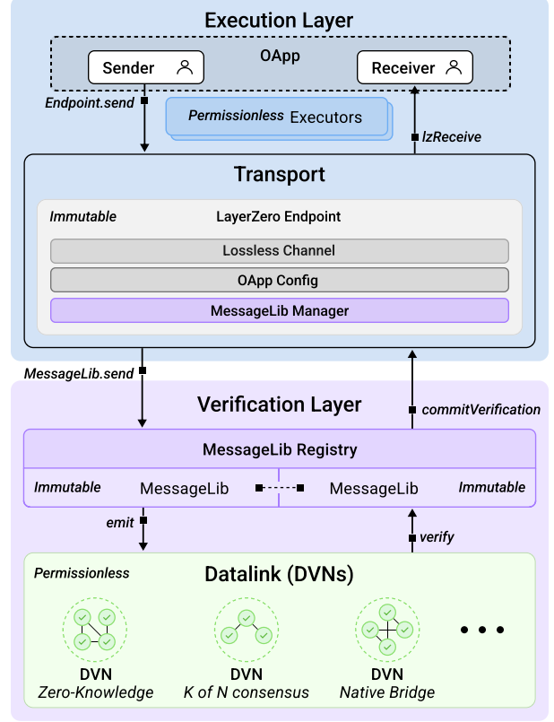
Figure 3: LayerZero is divided into execution and verification layers. The verification layer securely transmits data between blockchains, and the execution layer interprets this data to form a secure, censorship resistant messaging channel.
